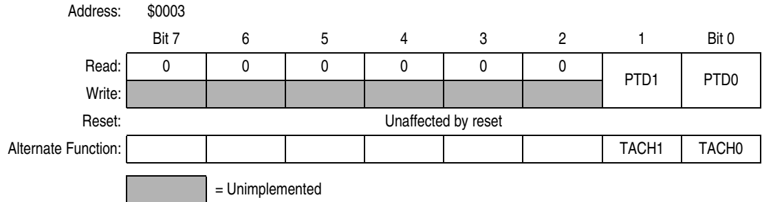
Figure 12-11. Port D Data Register (PTD)
