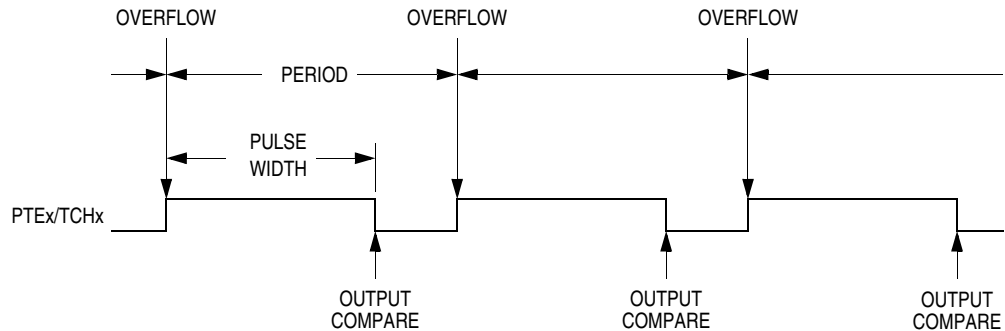
Figure 18-4. PWM Period and Pulse Width
