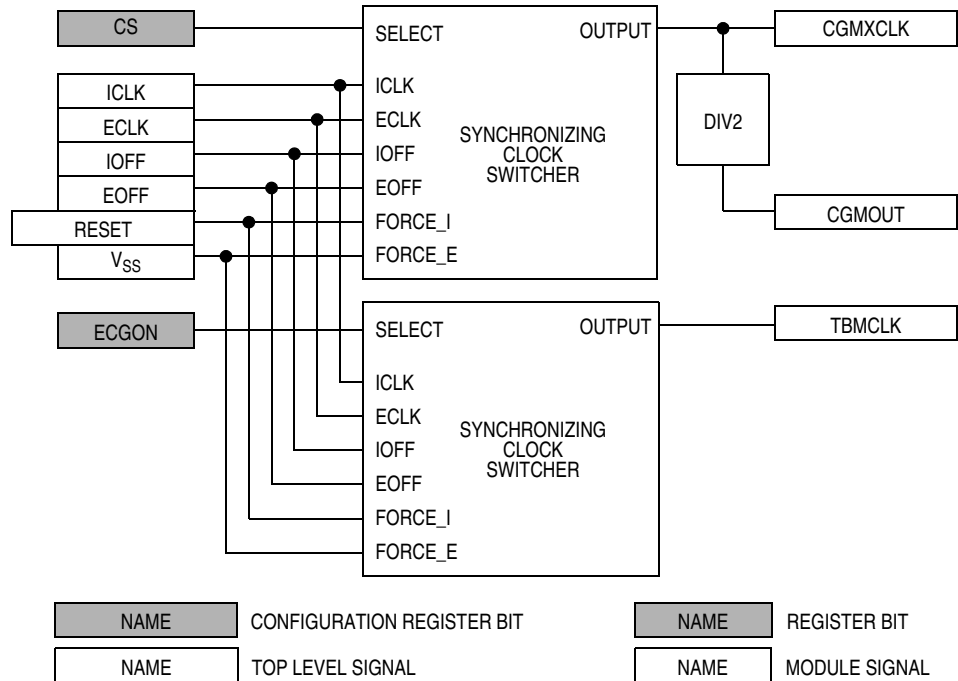
Figure 8-8. Clock Selection Circuit Block Diagram
