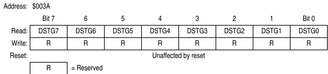
Figure 8-16. ICG DCO Stage Control Register (ICGDSR)
