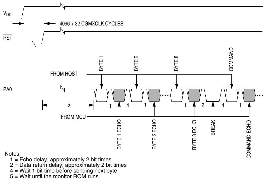
Figure 19-17. Monitor Mode Entry Timing
