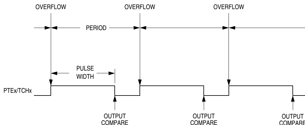
Figure 17-4. PWM Period and Pulse Width
