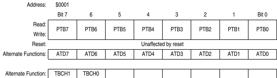
Figure 12-5. Port B Data Register (PTB)
