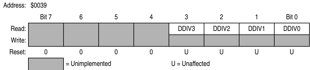
Figure 8-15. ICG DCO Divider Control Register (ICGDVR)
