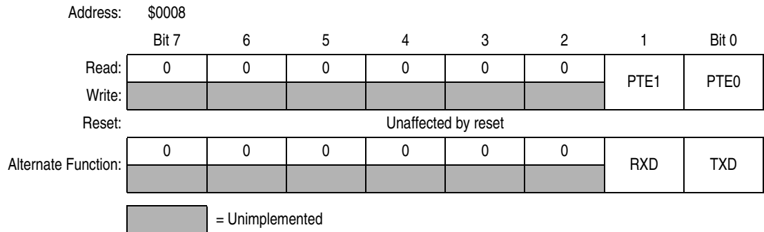
Figure 12-14. Port E Data Register (PTE)
