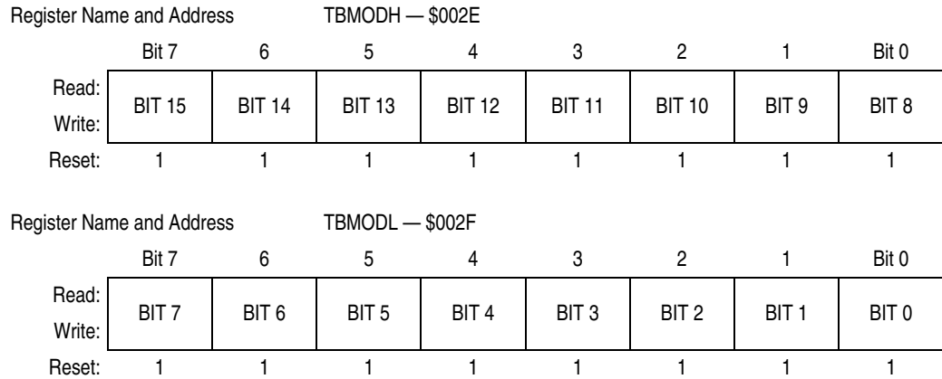
Figure 18-7. TIMB Counter Modulo Registers (TMODH and TMDL)
