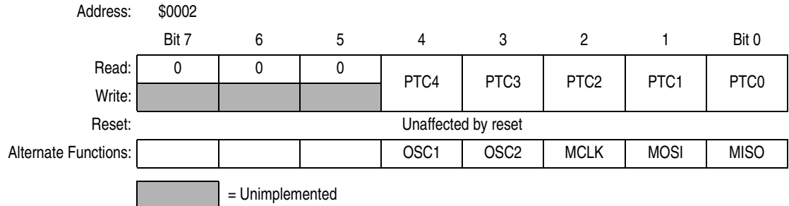
Figure 12-8. Port C Data Register (PTC)
