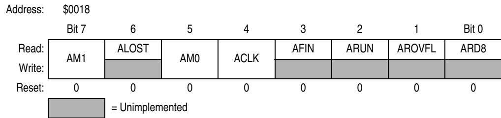
Figure 13-19. ESCI Arbiter Control Register (SCIACTL)
