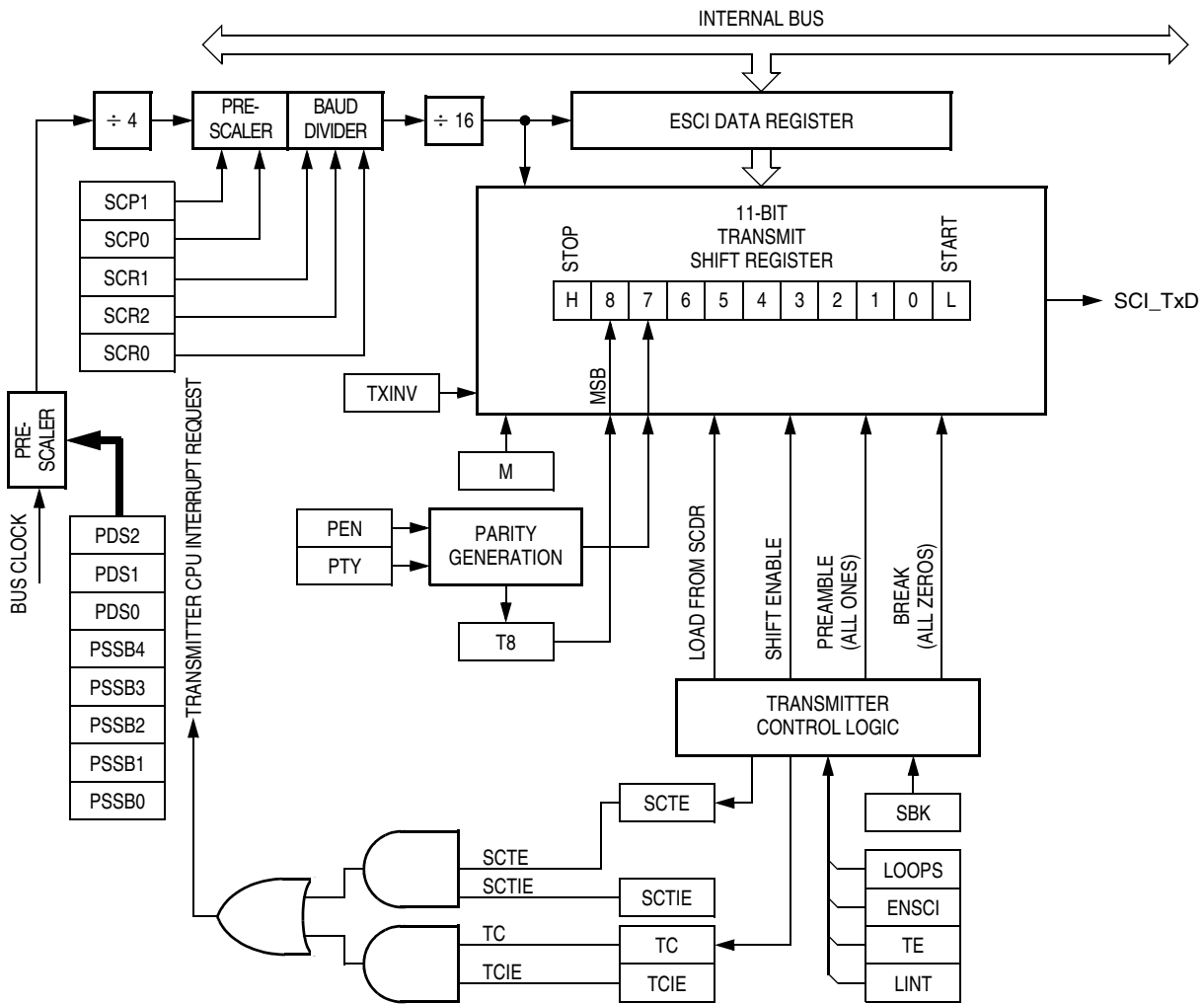
Figure 13-5. ESCI Transmitter
