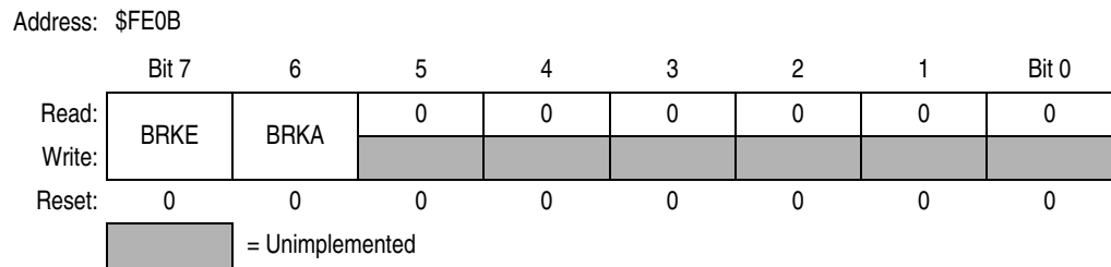
Figure 19-4. Break Status and Control Register (BSCR)
