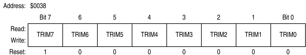
Figure 8-14. ICG Trim Register (ICGTR)
