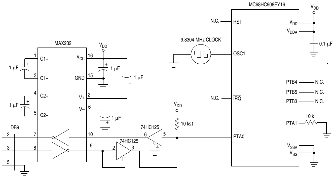
Figure 19-11. Forced Monitor Mode ( \overline{\text{IRQ}} = V_{DD} )
