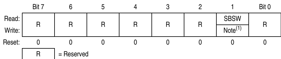
Figure 14-16. SIM Break Status Register (SBSR)
