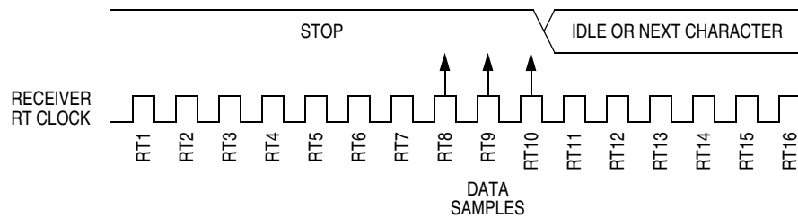
Figure 13-9. Fast Data
