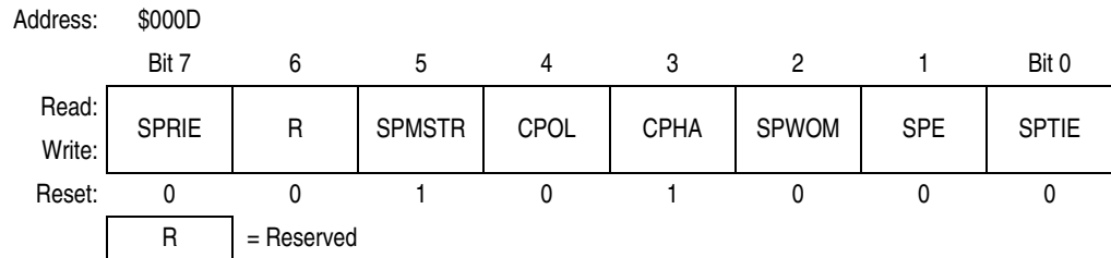
Figure 15-12. SPI Control Register (SPCR)
