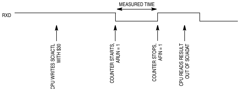
Figure 13-23. Bit Time Measurement with ACLK = 1 , Scenario B
