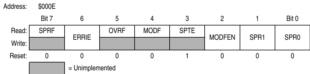
Figure 15-13. SPI Status and Control Register (SPSCR)
