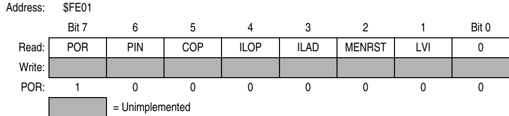
Figure 14-17. SIM Reset Status Register (SRSR)
