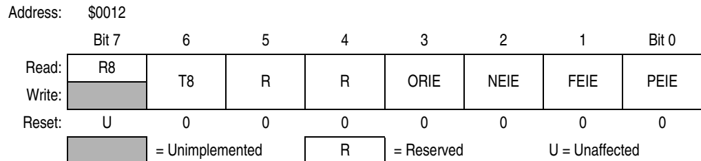
Figure 13-12. ESCI Control Register 3 (SCC3)
