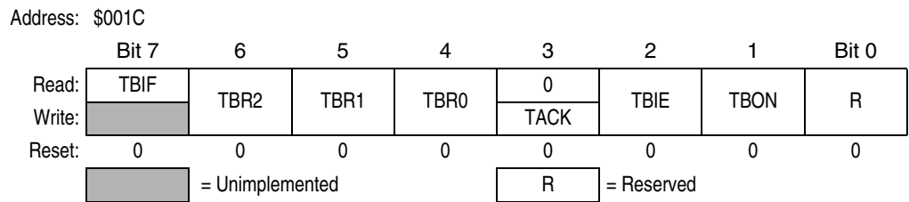
Figure 16-2. Timebase Control Register (TBCR)
