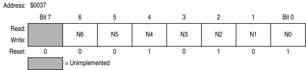
Figure 8-13. ICG Multiplier Register (ICGMR)
