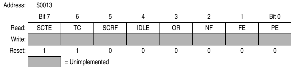
Figure 13-13. ESCI Status Register 1 (SCS1)
