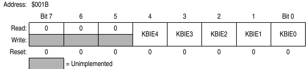
Figure 10-5. Keyboard Interrupt Enable Register (KBIER)
