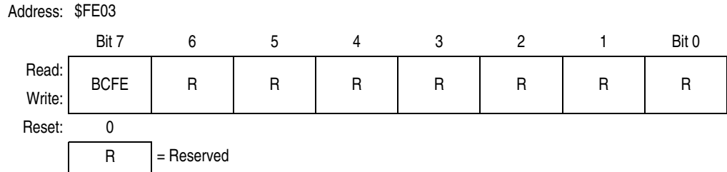
Figure 19-8. Break Flag Control Register (SBFCR)
